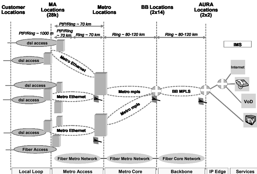
Figure 1 - Overview of KPN's planned ALL-IP network
